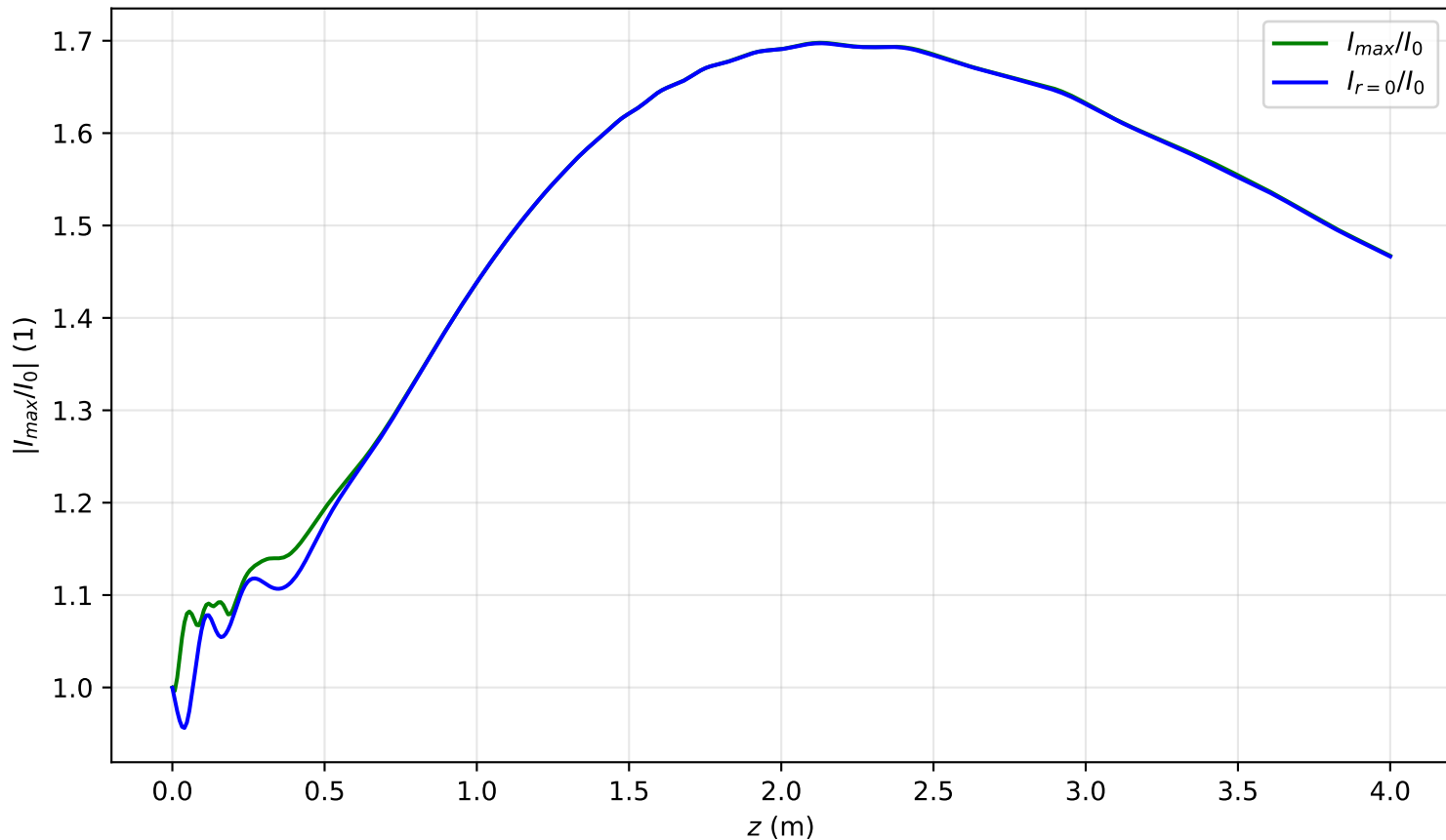
I_{max}(x = 0, y = 0, z)/I_0 , P_{in}=0.9P_{cr} , noisy input, artificial time
